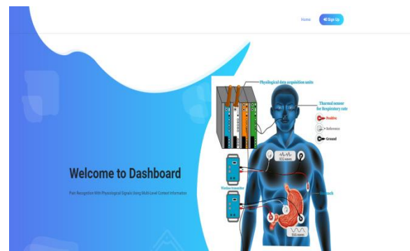
Fig 12 Home page
