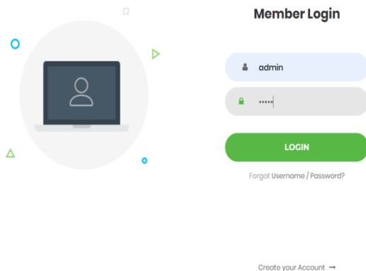
Fig 14 Login page
