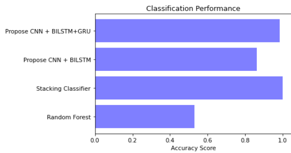
Fig9 Accuracy graph
