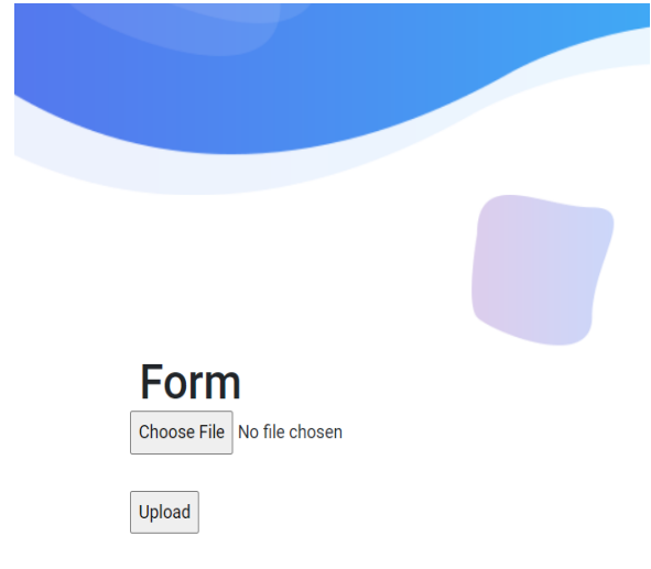
Fig 15 User input
